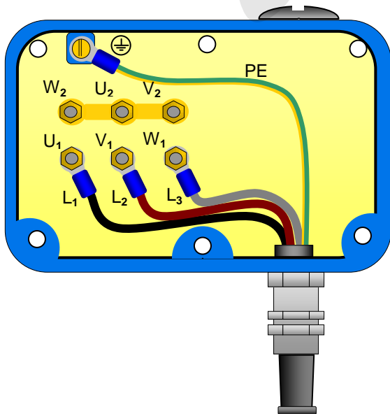
Figure 5 G5x/GE5x Terminal box allocation 3 ~ 400 V / Y- switching
