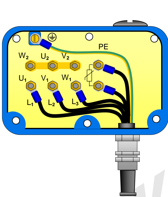
Figure 4 G5x/GE5x Terminal box allocation 3 ~ 400 V / Y- switching, with thermal protector Thermistor PTC 120
