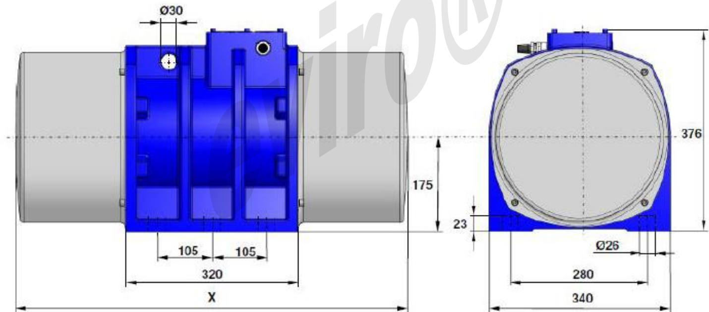
Figure 3 Motor dimensions G51/GE51 series
