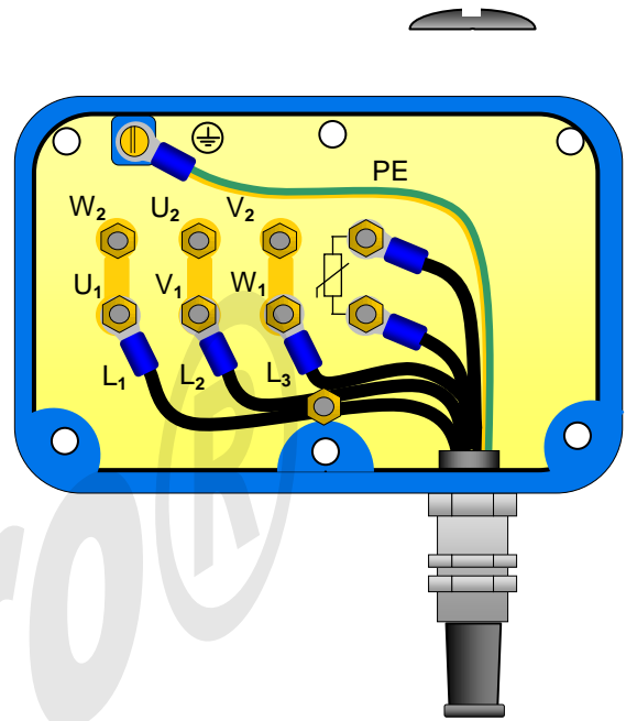
Figure 6 G5x/GE5x Terminal box allocation 3 ~ 230 V / Δ- switching, with thermal protector Thermistor PTC 120
