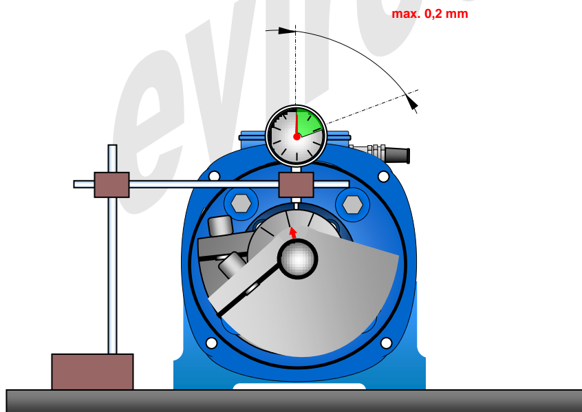
Figure 11 G40/GE40 Verifying radial clearance
