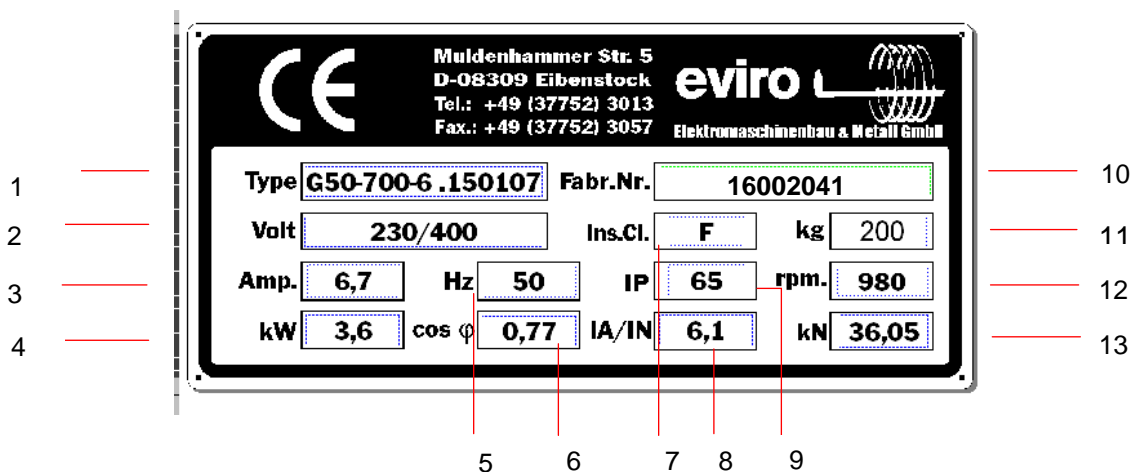
Figure 1 Type plate
