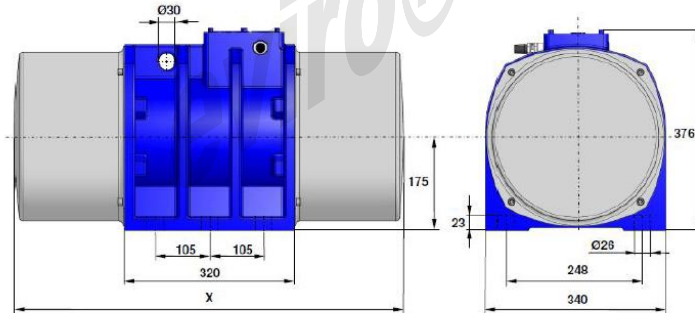
Figure 2 Motor dimensions G50/GE50 series
