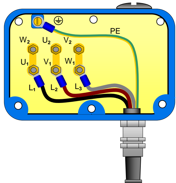
Figure 7 G5x/GE5x Terminal box allocation 3 ~ 230 V / Δ- switching
