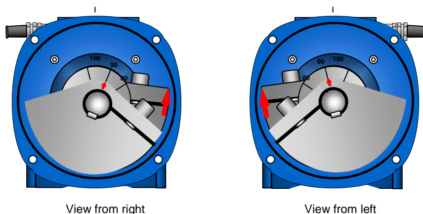
Figure 7 G32 Adjustment of centrifugal force
