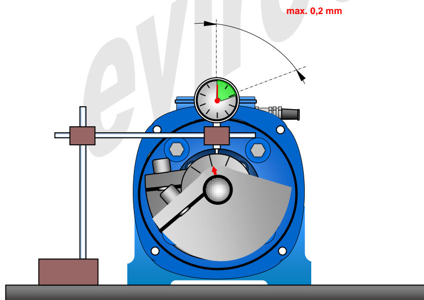
Figure 8 G32 Verifying radial clearance
