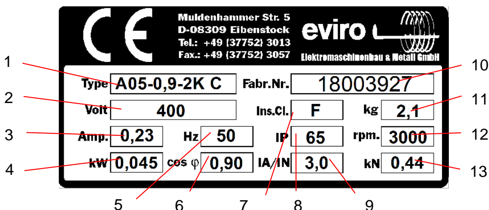
Figure 1 Type plate
