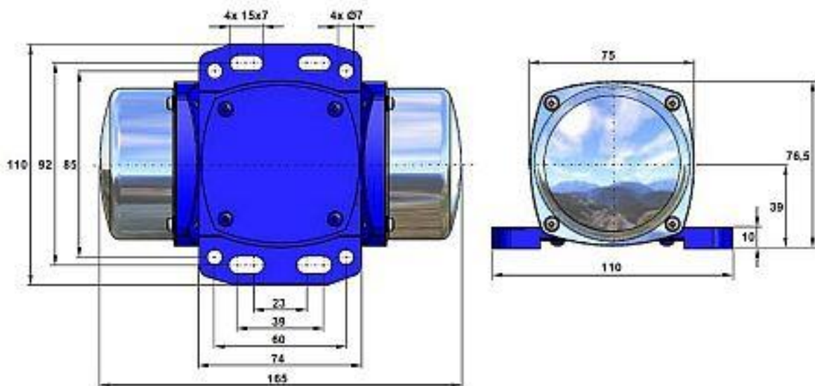
Figure 2 Motor dimensions
